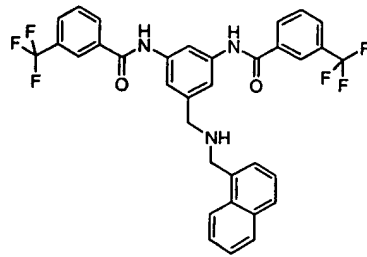
Compound # 14
